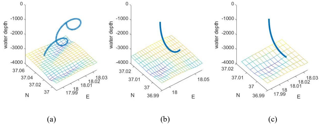
Figure 5. Submarine trajectories at different initial velocities (a) v_z = 0.1 \text{ m/s} (b) v_z = 0.4 \text{ m/s} (c) v_z = 0.7 \text{ m/s}
