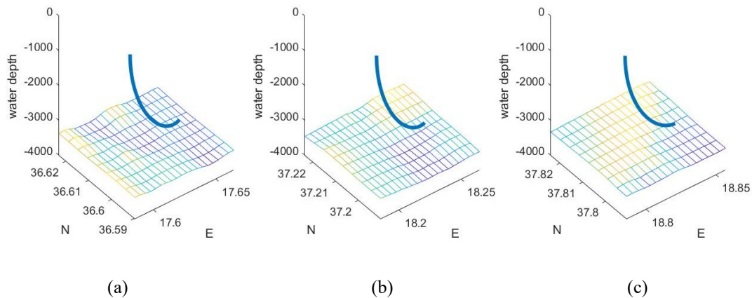
Figure 6. Submarine trajectories at different incident locations (a) 36.6^\circ \text{N } 17.6^\circ \text{E} (b) 37.2^\circ \text{N } 18.2^\circ \text{E} (c) 37.8^\circ \text{N } 18.8^\circ \text{E}
