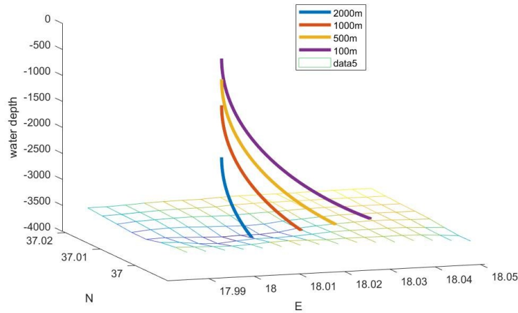
Figure 4. Trajectory prediction considering real ocean currents
