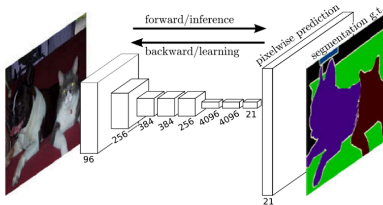
Figure 1. FCN semantic segmentation network model [4]
