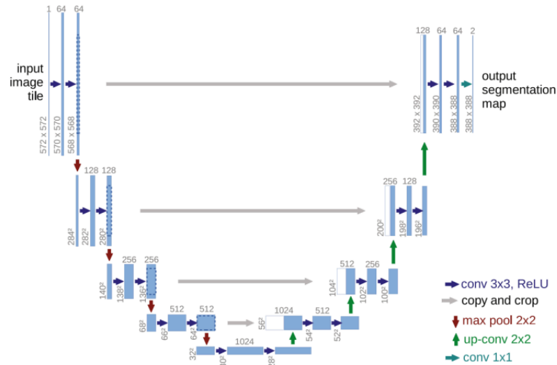
Figure 2. U-Net semantic segmentation network model [5]
