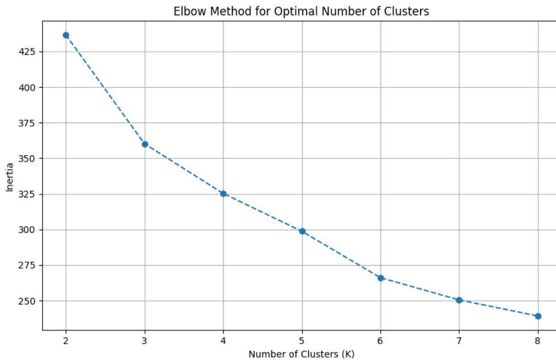
Figure 1. Relationship Between Number of Clusters and SSE
