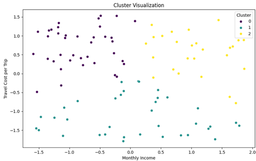
Figure 2. Clustering Results Visualization
