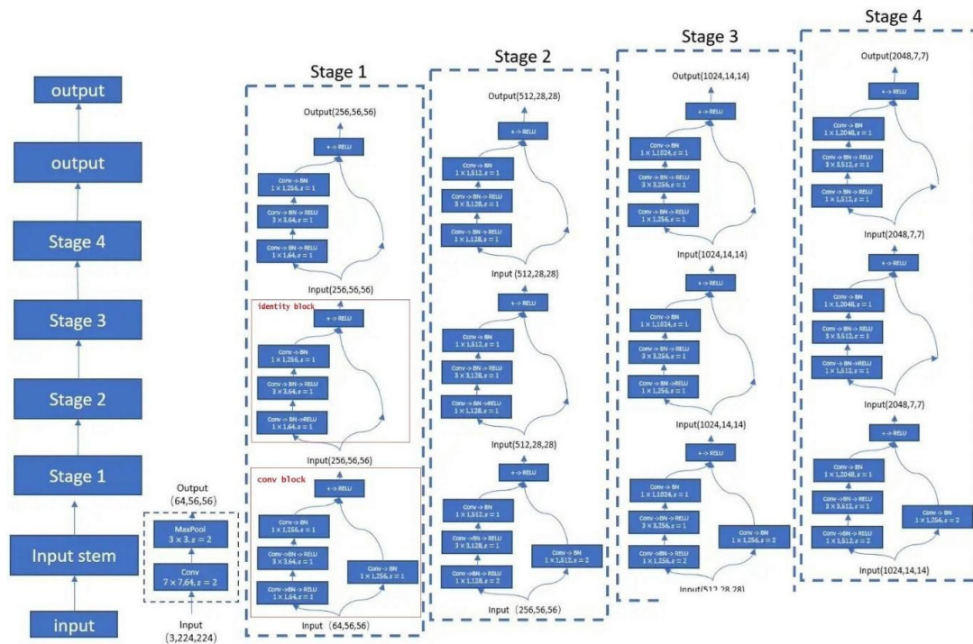
Figure 3. Resnet-50 structure [1]
