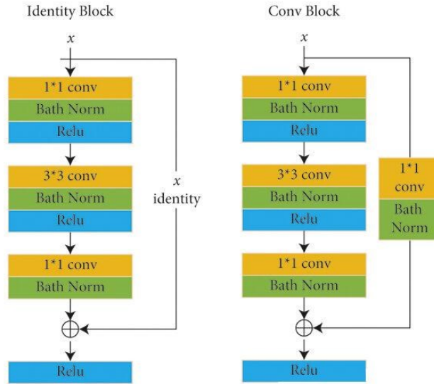
Figure 4. Structure of Identity Block and Convolutional Block
