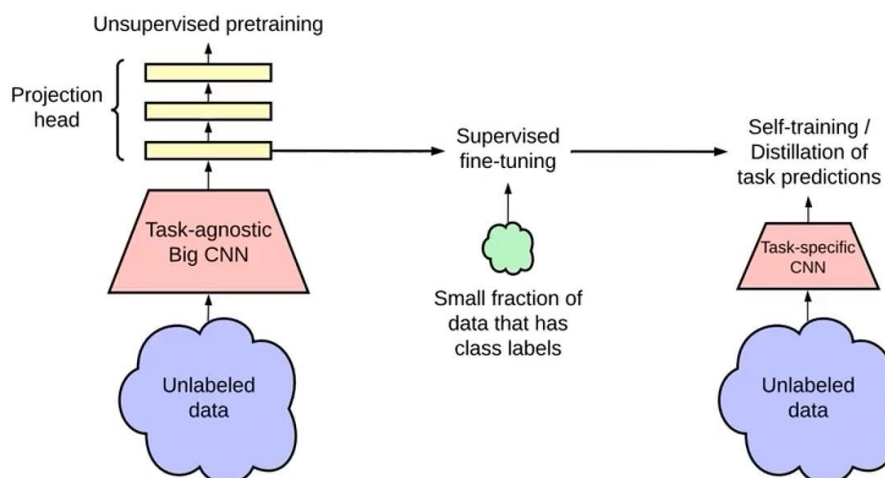
Figure 9. Unsupervised learning, Contrastive learning
