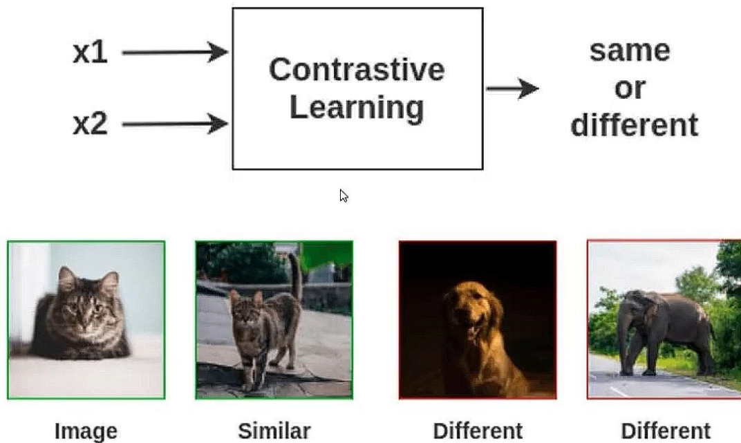
Figure 6. Contrastive learning
