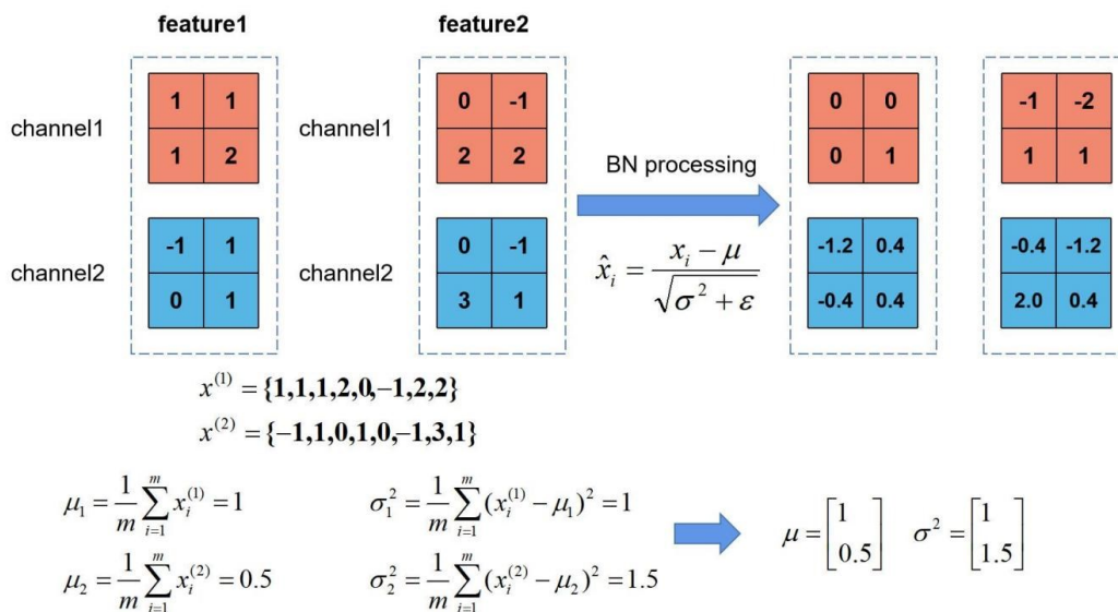
Figure 5. Logic of Batch Normalization Layers
