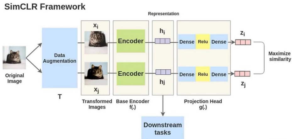
Figure 8. Logic of contrastive learning [4,5]
