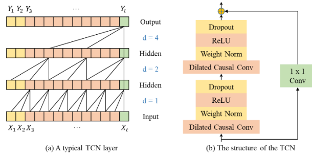
Figure 3: Time convolutional network
