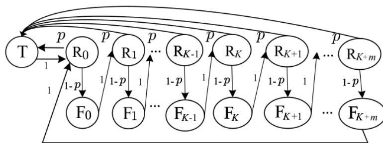
Figure 1. Markov chain
